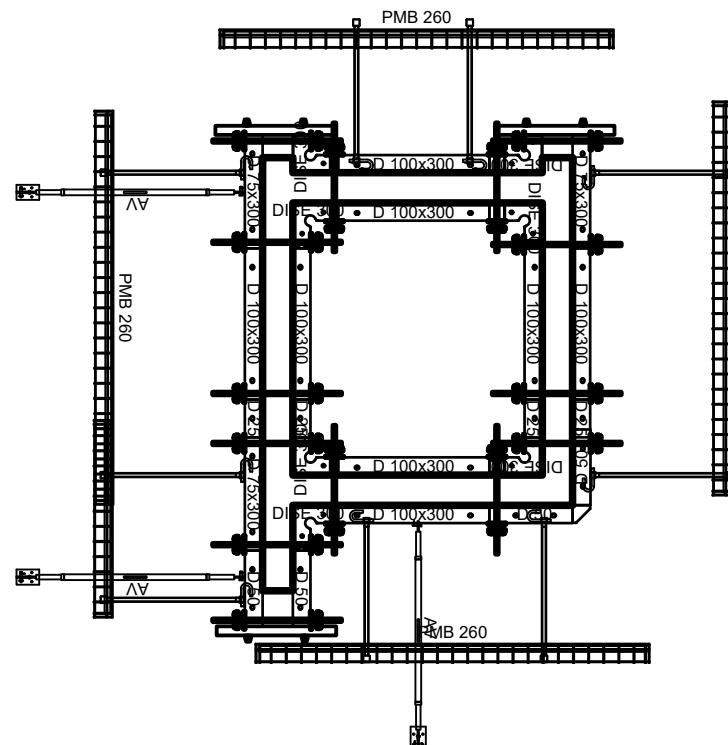
PLAN OPLATE - TAKT 1
