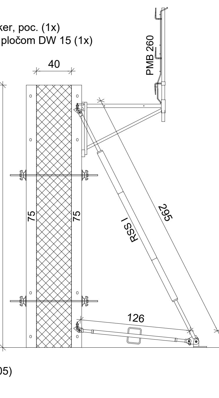
Presek 2-2 1:25
