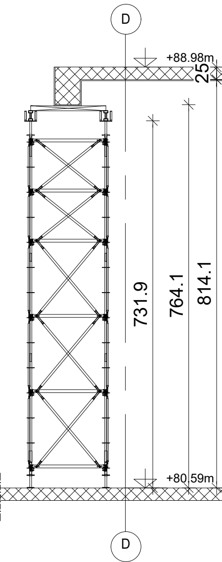
Section 2-2 - part I 1:75
