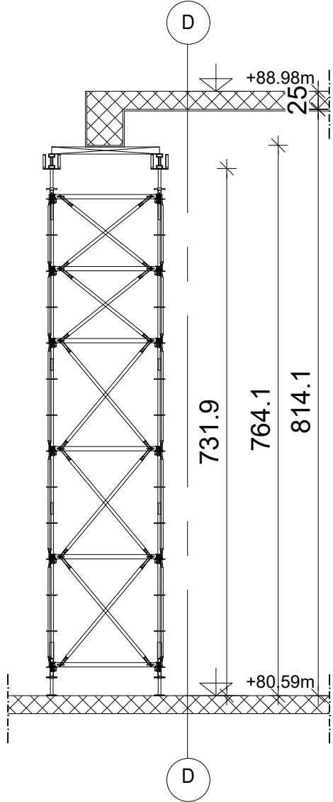
Section 2-2 - part I 1:75
