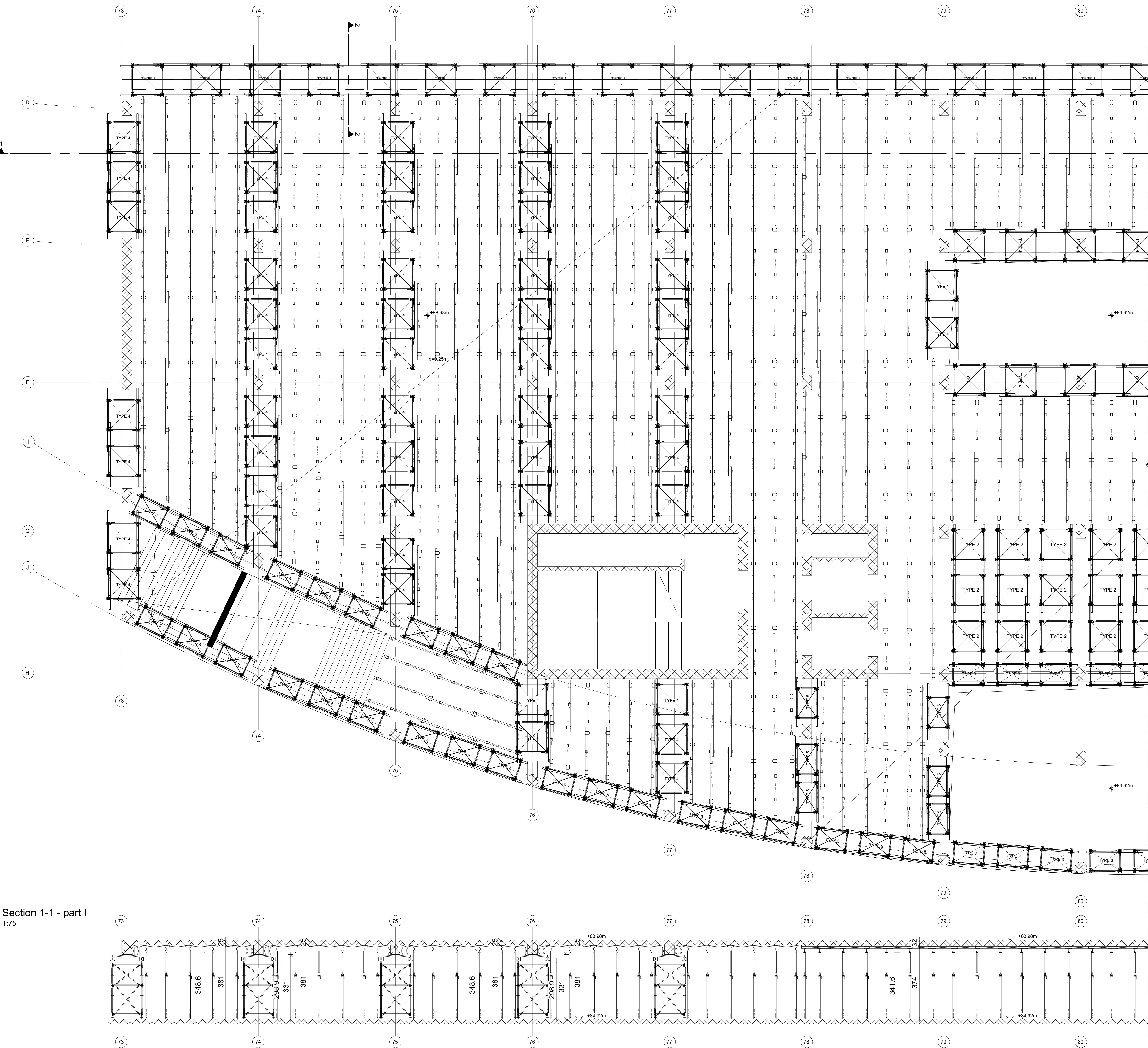
Formwork plan - part I 1:75
