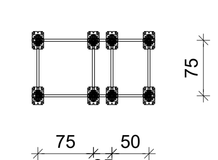
Tower Type 111 1:50
