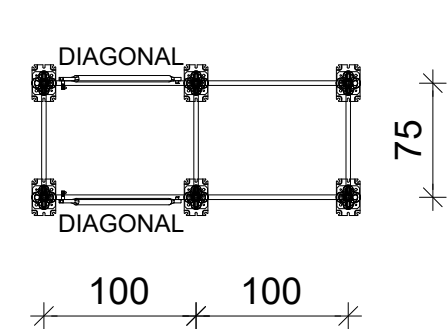
Tower Type 101 1:50
