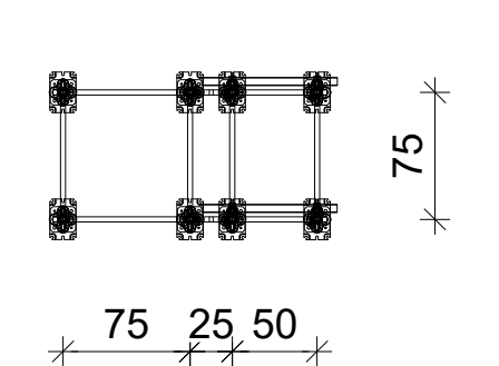
Tower Type 105 1:50
