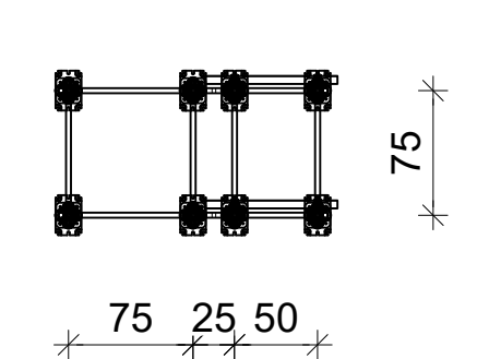
Tower Type 107 1:50
