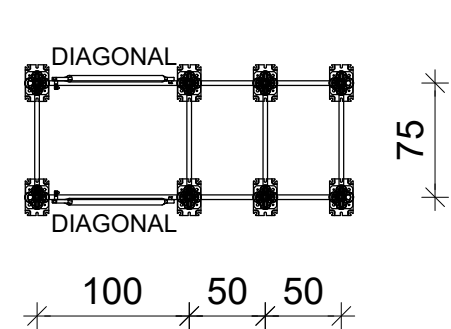
Tower Type 103 1:50
